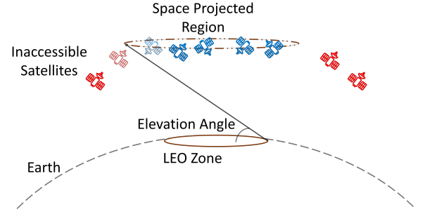
Figure 3: Defining the space projected region for a LEO zones based on elevation angle constraints.
