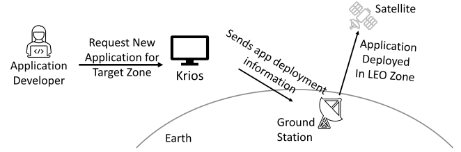
Figure 6: Workflow of application deployment in Krios.
