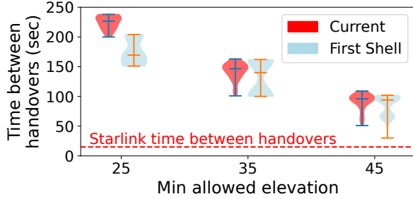
Figure 10: Comparing time between handovers for different minimum elevation angle constraints using Krios. Starlink currently uses a constant 15 second handover interval.
